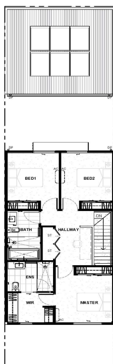
First floor
