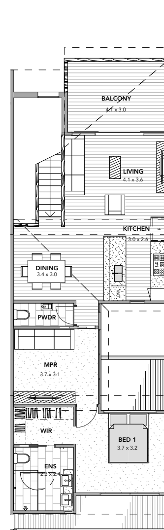
First floor
