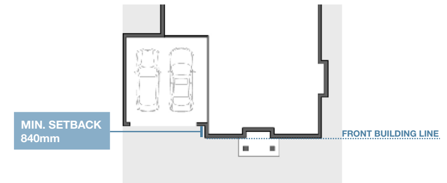
Garage Setback
