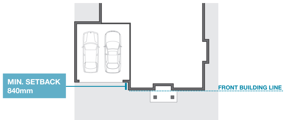
Garage Setback
