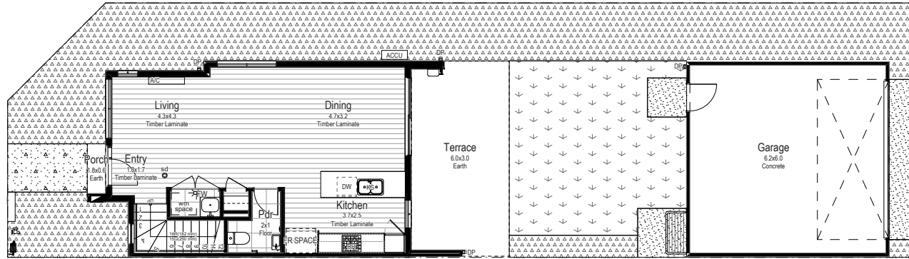
Ground Floor
