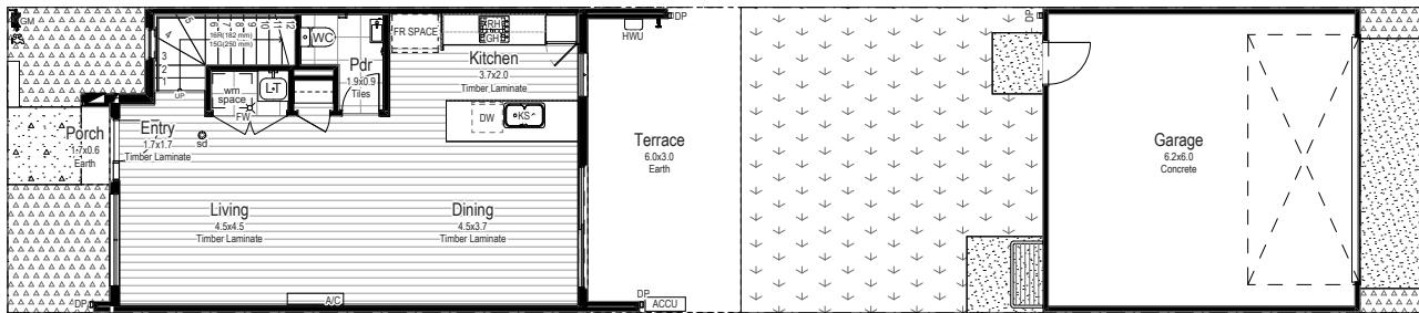
Ground Floor
