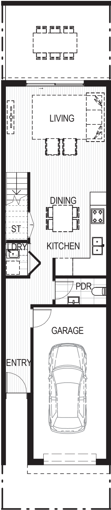
GROUND FLOOR PLAN
